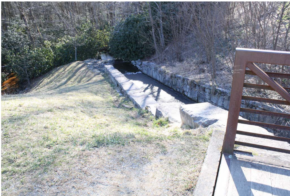
Plate 11.4: Spillway at Sims Pond Dam (WT0957), from the south end of the bridge.
