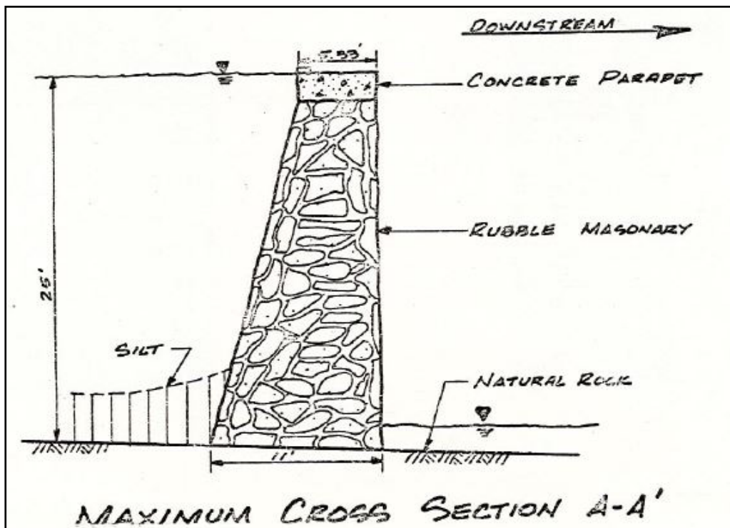
Figure 2.5: Sloop's Dam cross section (from AV0082 HPO survey file, drawn by Golder and Associates, 1980).
